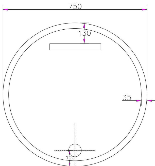
Mounting Base Detail
