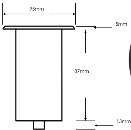
Cut-Out Fitting Only 65mm
