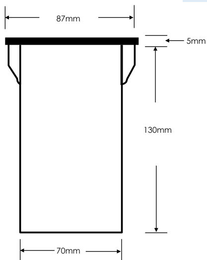
Cut-Out With Can 87mm
