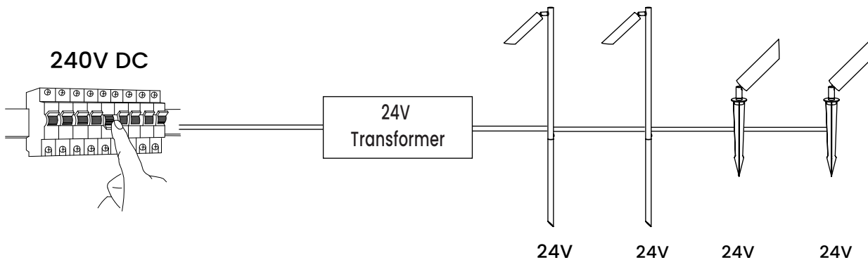
Transformer 60W 24V IP68 C TR060.24V IP68
