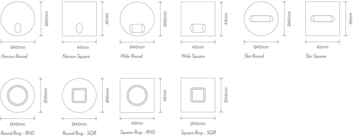
LED Module
