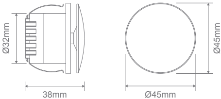
Cut-out: Ø35mm
